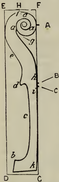
FIG. 161.—Plank outline of Neck and Scroll (on block).
